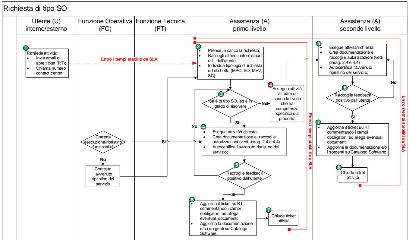
Figura 4: Workflow SO
