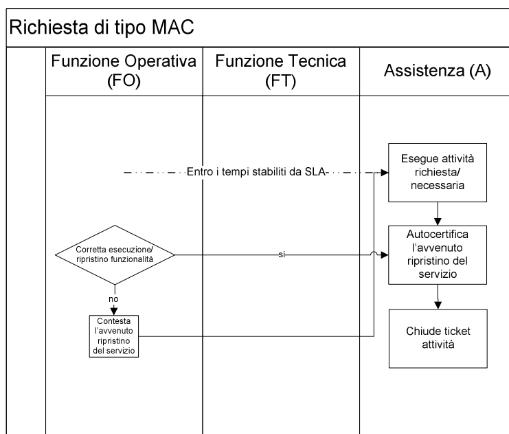
Figura 1: Workflow MAC
